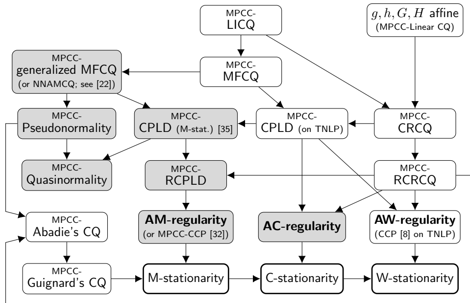
FIG. 2. Relations between CQs for MPCCs. Shaded balloons are those CQs that have an explicit restriction of C- or M-stationarity type. The arrows between CQs indicate logical implications. The arrows pointing to stationarity balloons represent those stationarity concepts guaranteed by a CQ at minimizers of (MPCC).
